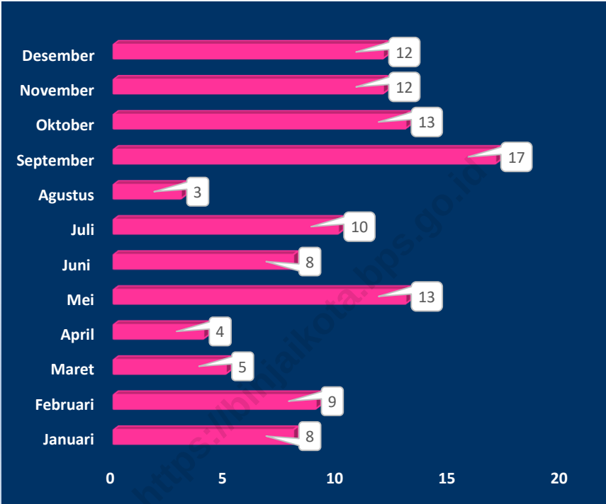
Gambar 1.1 Perbandingan Hari Hujan di Kecamatan Binjai Kota, 2019 Picture Comparison of Rain Days in Binjai Kota Sub district 2019
