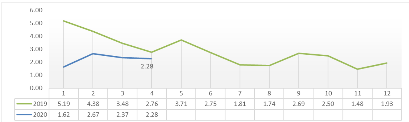
Series Inflasi year-on-year
