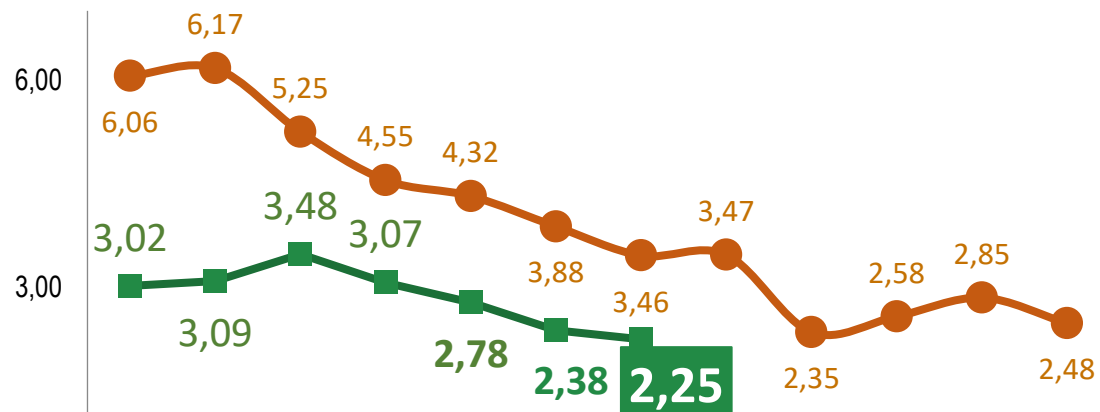
Series y-on-y
