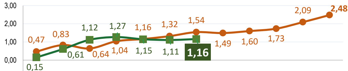
Series Y-to-D
