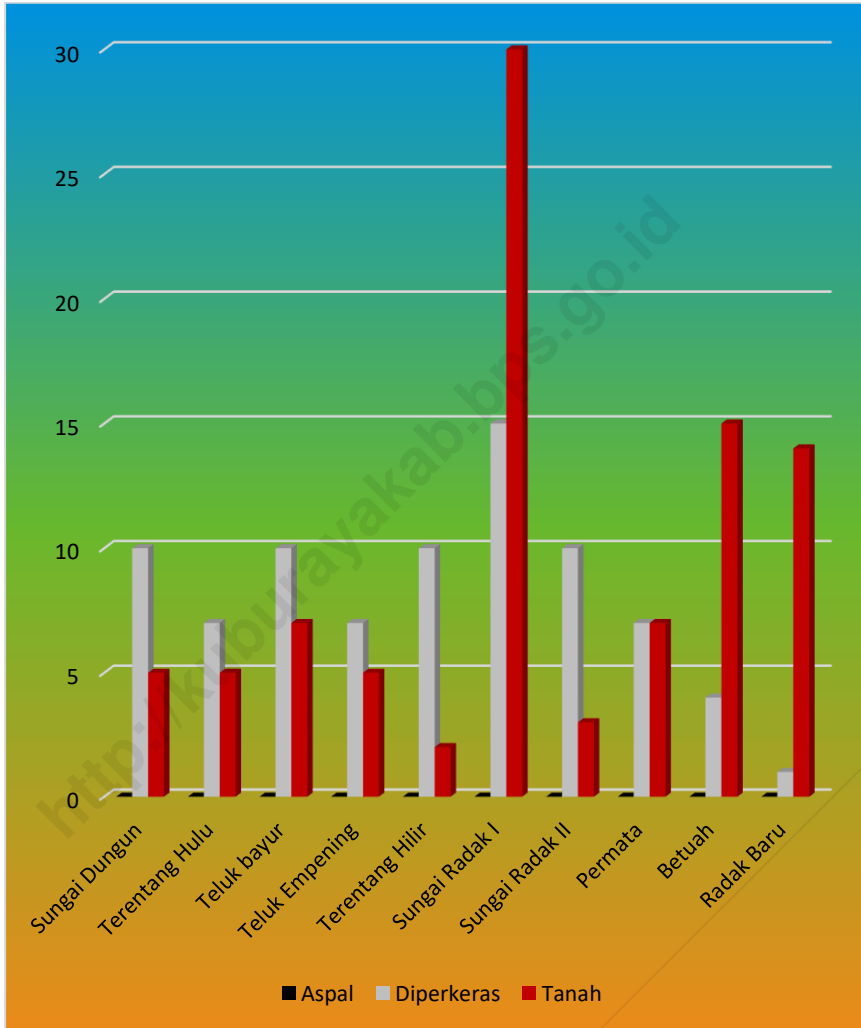
Grafik 8. Panjang Jalan menurut desa dan Jenis Permukaan di Kecamatan Terentang (KM) Length of Road by Village and Surface Type in Terentang District (KM)
