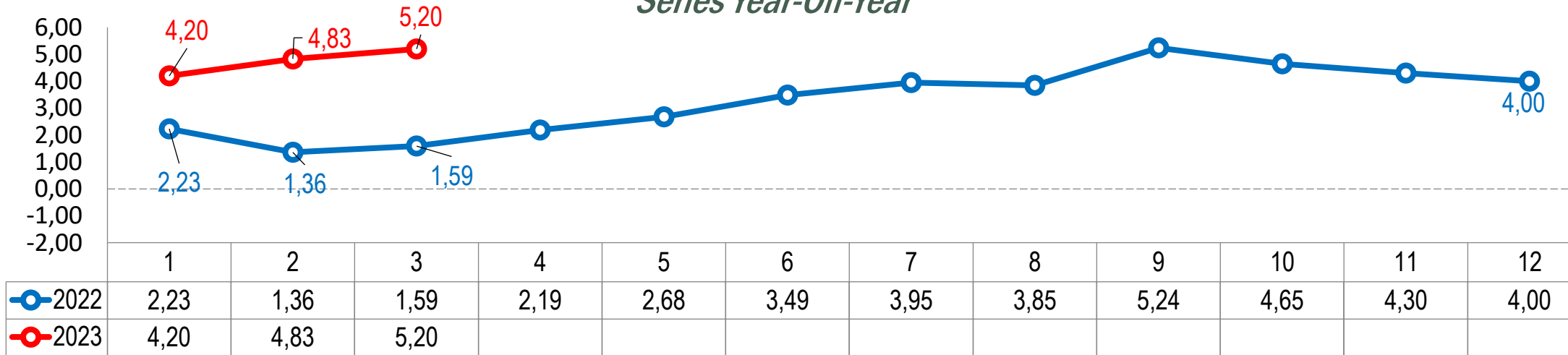
Series Year-On-Year
